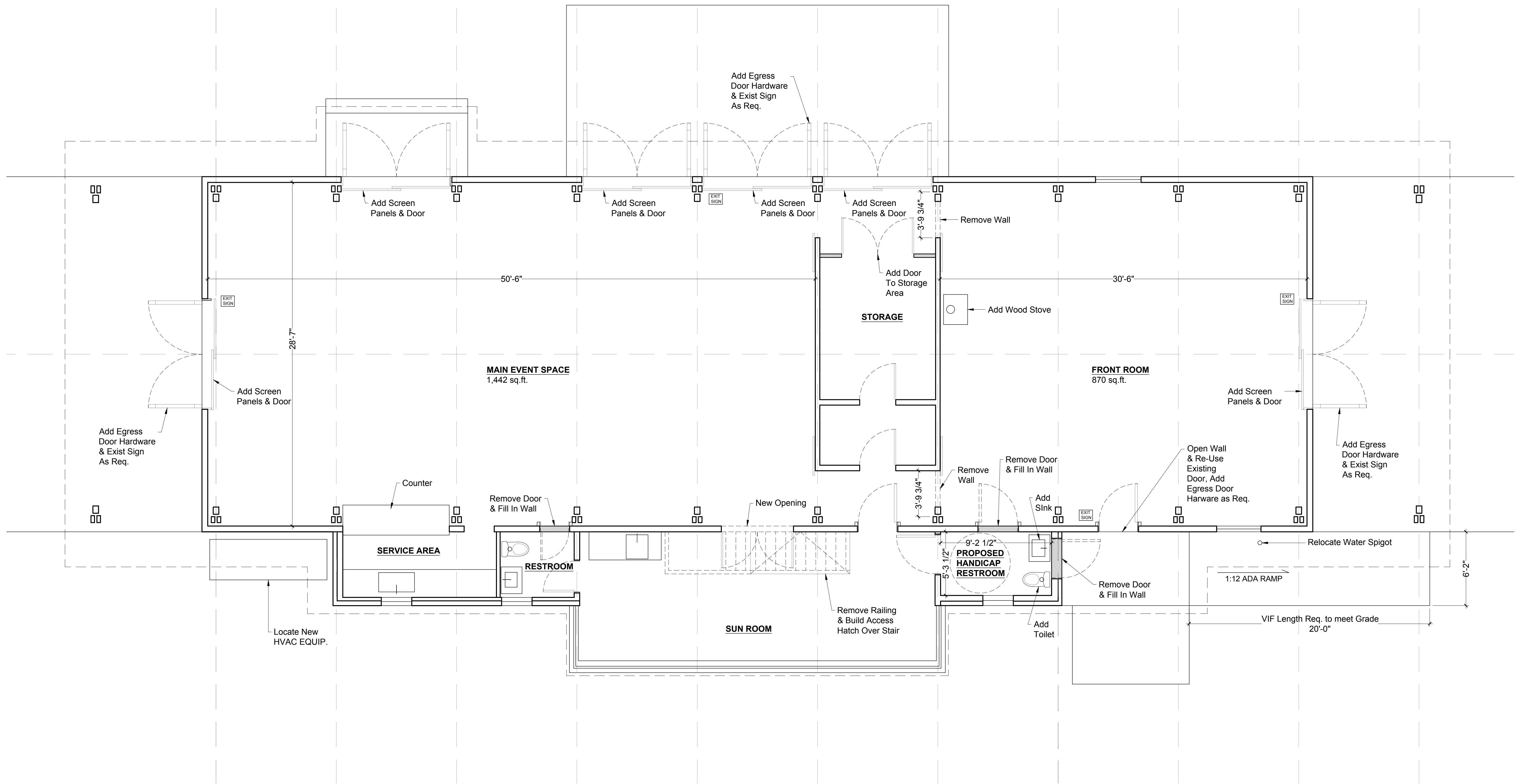
1 First Floor Plan Scale 1/4" = 1'-0"
