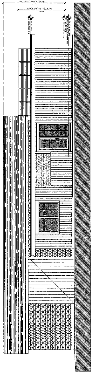
1 EAST - GUEST HOUSE ELEVATION SCALE: 1/8" = 1'-0"
