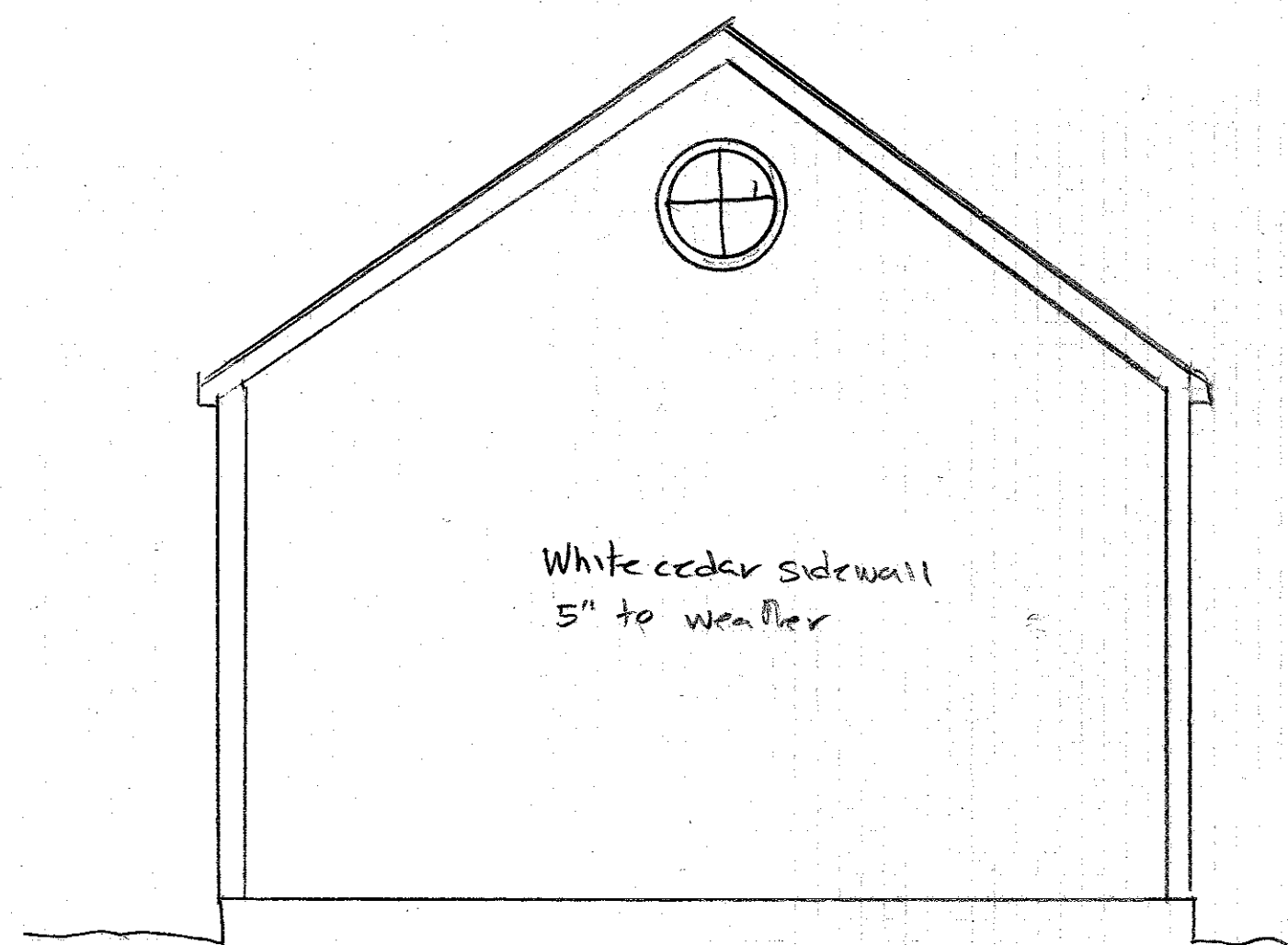
Halperin Studio East elevation 1/4" = 1' 10/28/20
