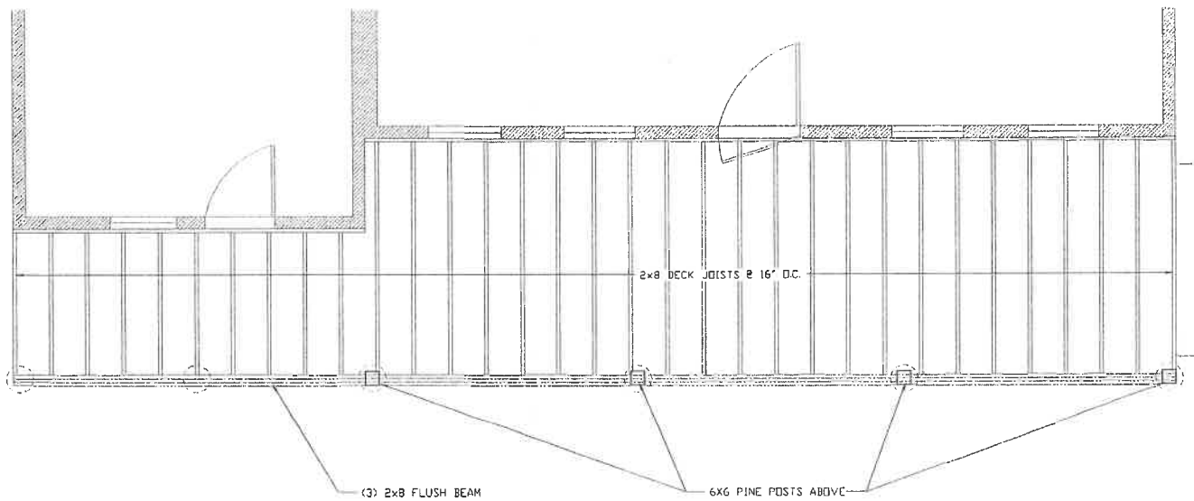
2 PORCH FLOOR FRAMING PLAN SCALE: 1/4"=1'-0"
