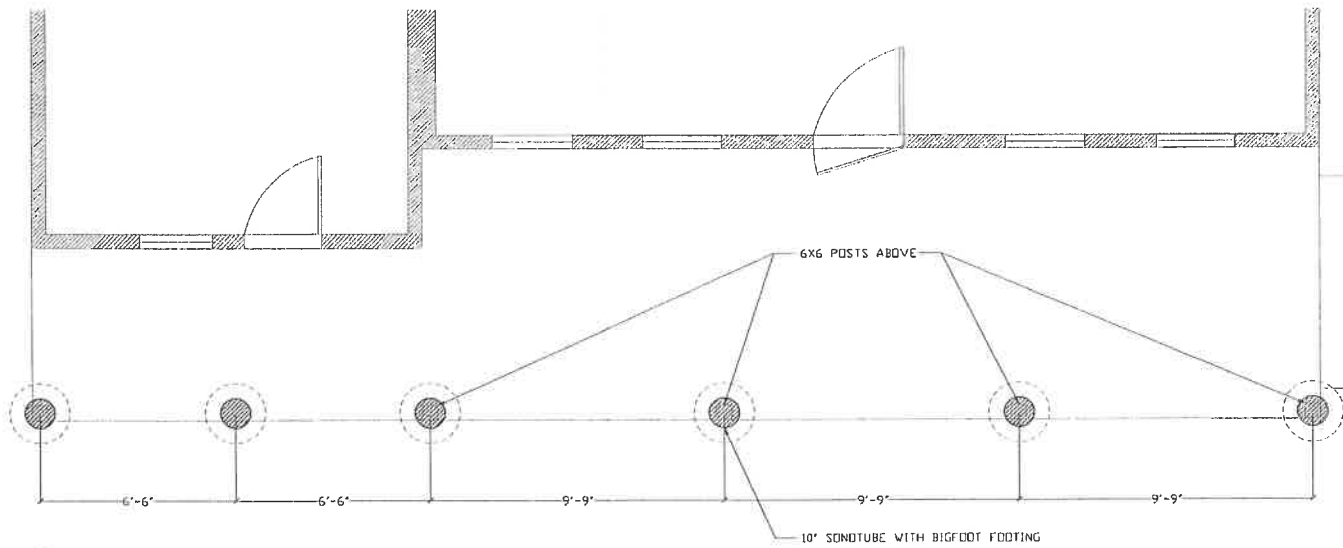
1 PORCH FOUNDATION PLAN SCALE: 1/4"=1'-0"
