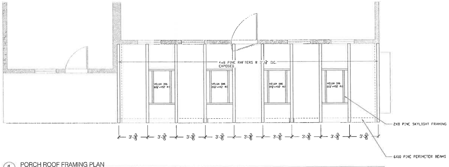
1 PORCH ROOF FRAMING PLAN SCALE: 1/4" = 1'-0"
