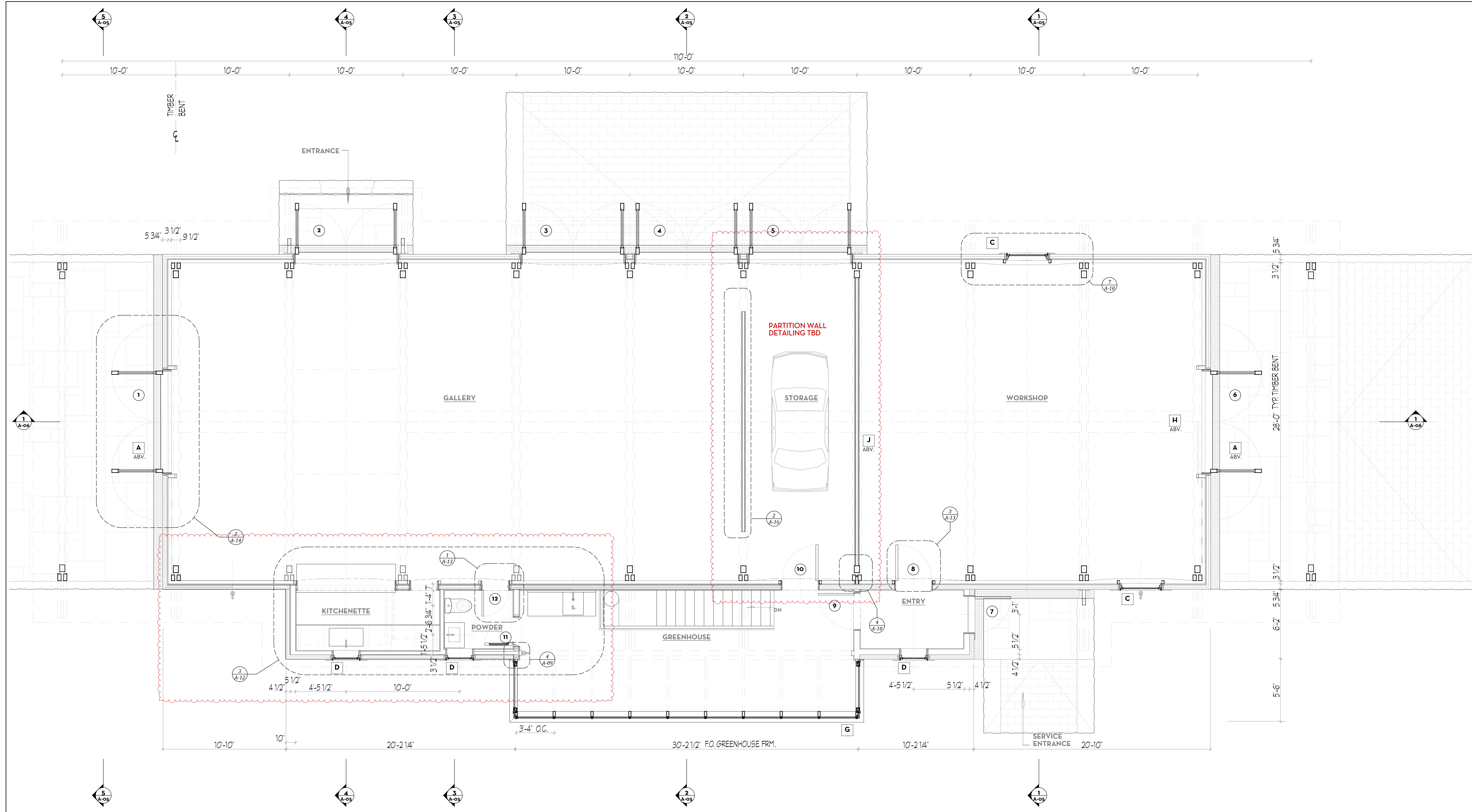
1 GROUND FLOOR PLAN SCALE: 1/4" = 1'-0"
