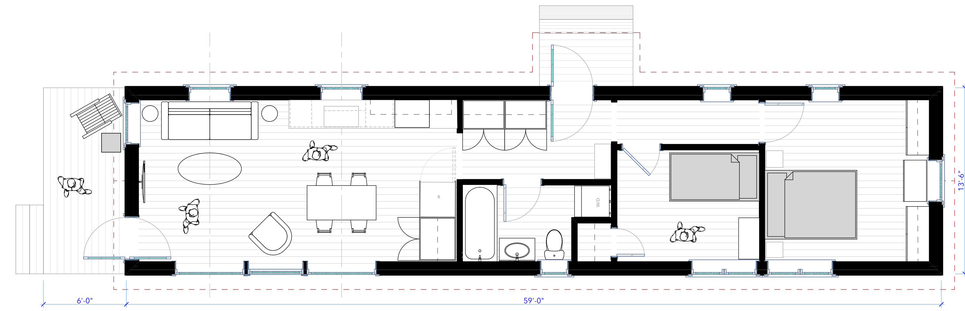
5 HOUSE #1+2 FIRST FLOOR PLAN SCALE: 1/4" = 1'-0"
