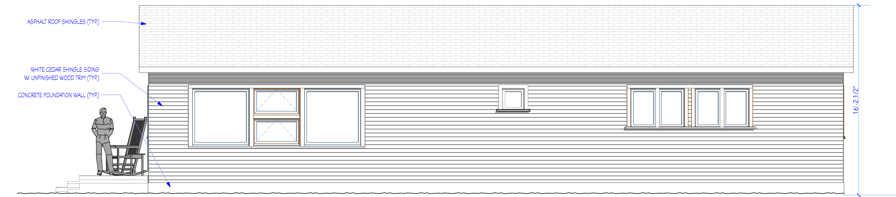
4 HOUSE 1+2 SOUTH ELEVATION SCALE: 1/4" = 1'-0"
