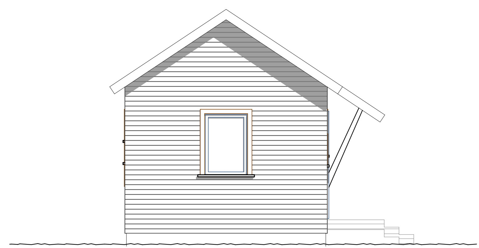
1 HOUSE 1+2 EAST ELEVATION SCALE: 1/4" = 1'-0"
