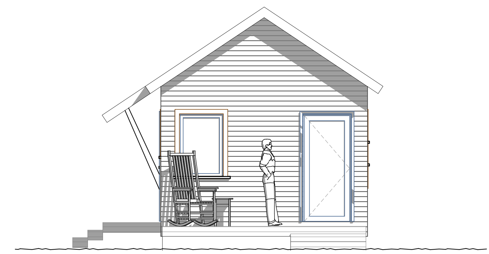
3 HOUSE #12 WEST ELEVATION SCALE: 1/4" = 1'-0"
