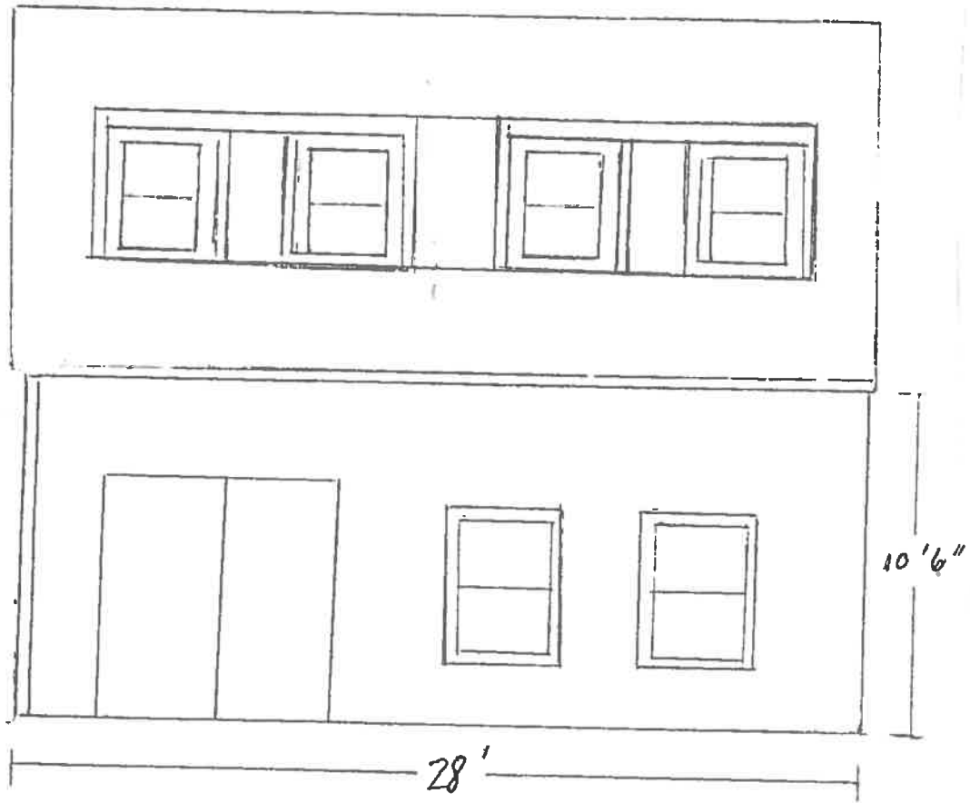
North Elevation
