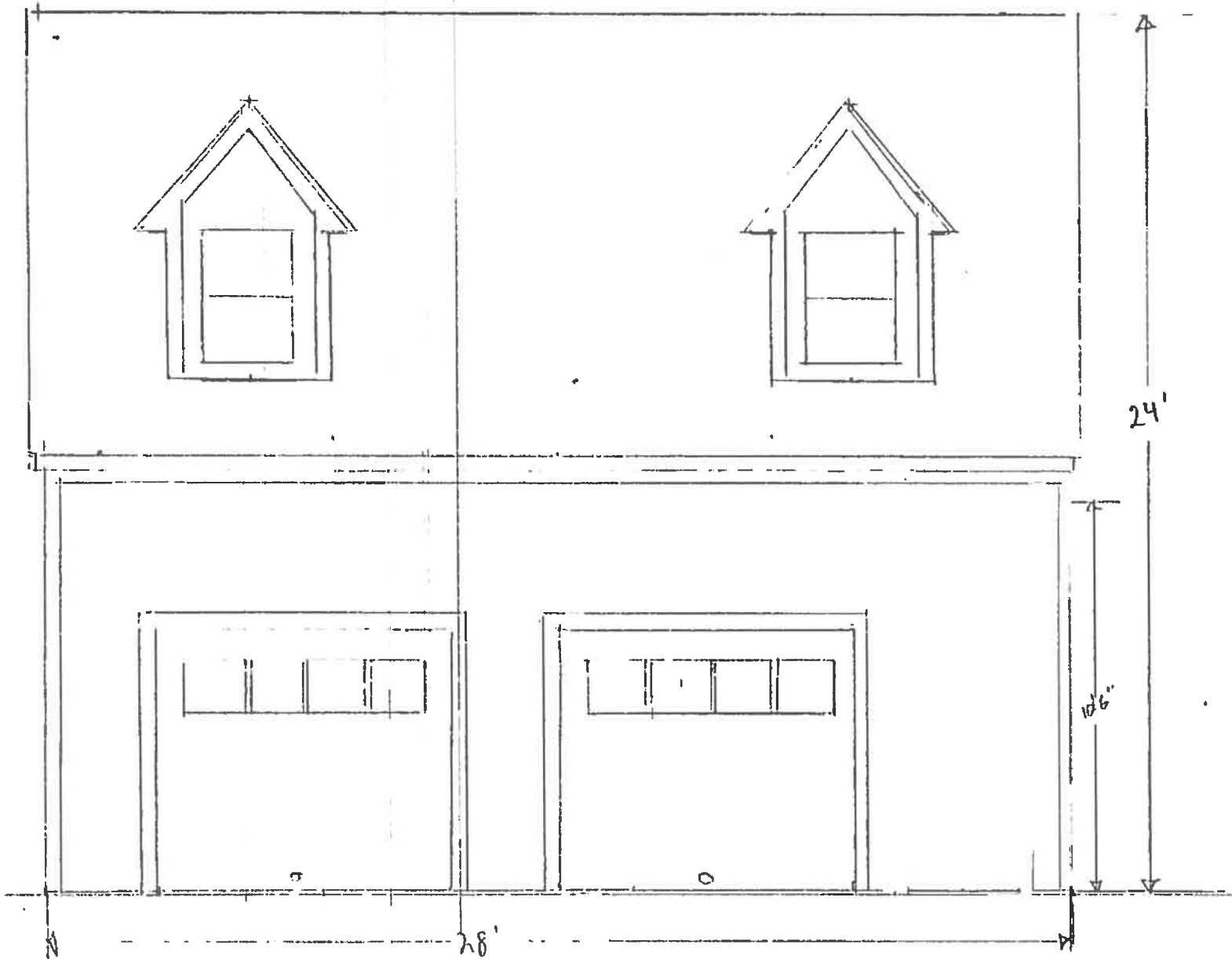
South Elevation
