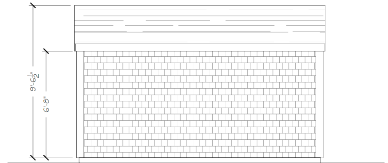
BACK ELEVATION
