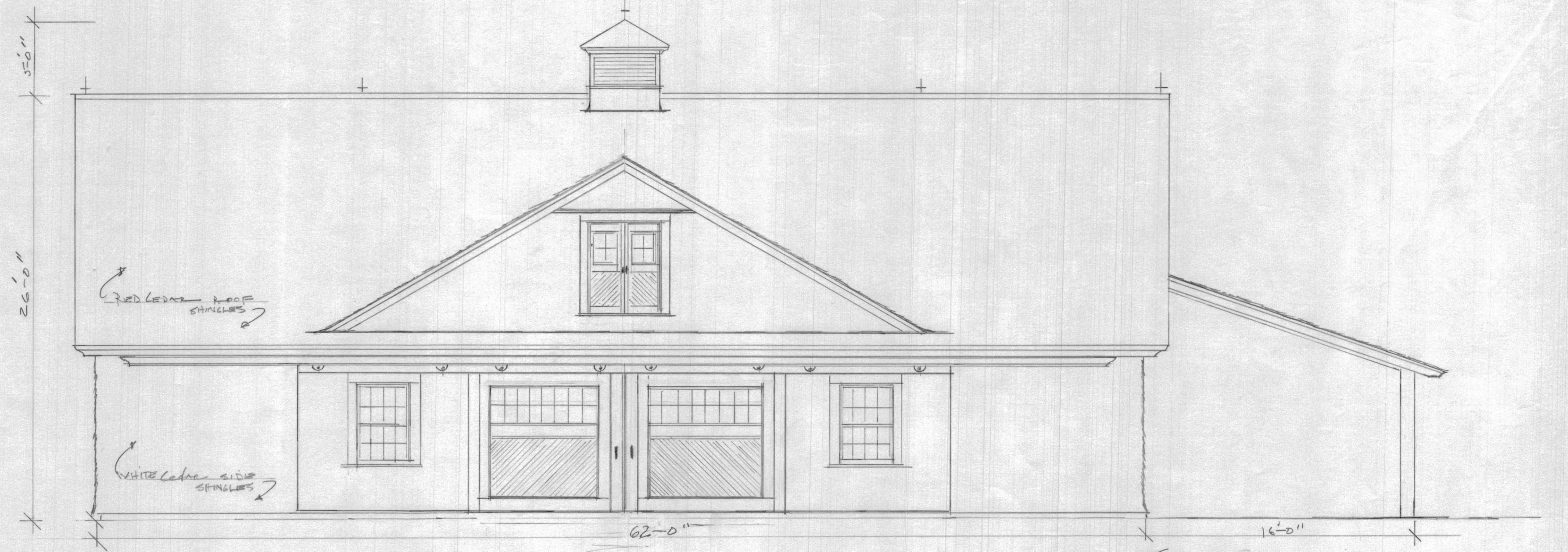
SOUTH ELEVATION 1/4" SCALE
