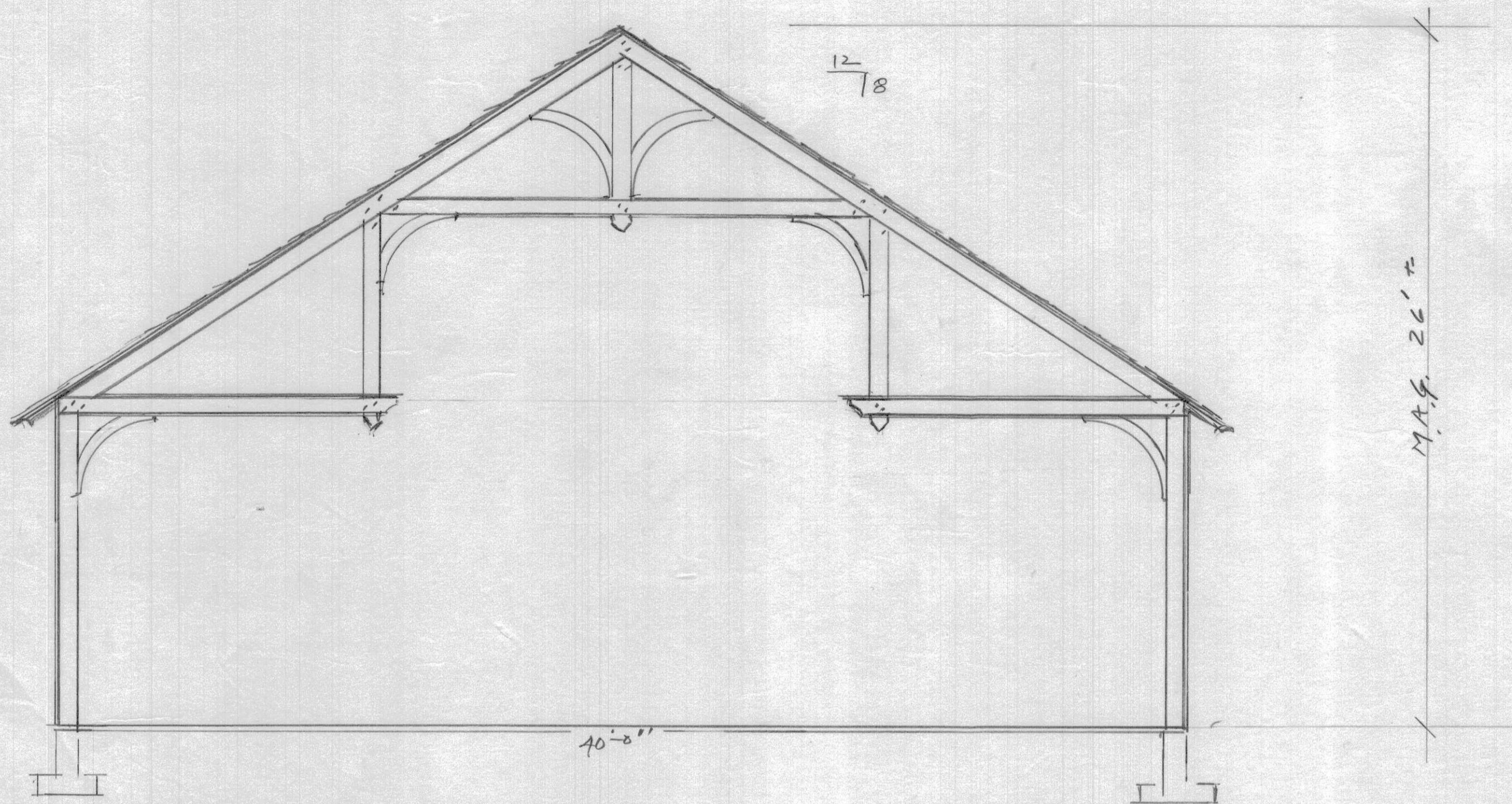
POST & BEAM SECTION 1/4 SCALE
