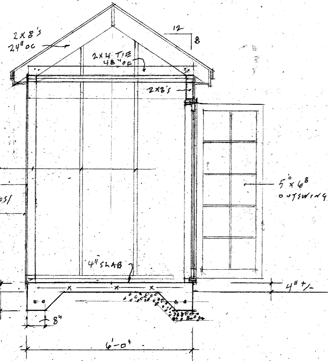
SECTION 1/2" = 1'-0"
