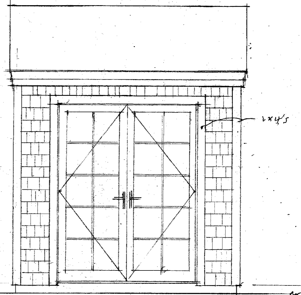
FRONT ELEVATION 1/2" = 1'-0" 8'-0"
